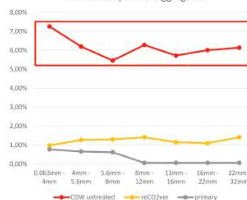
Water absorption of aggregates
